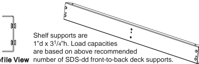
Profile View
